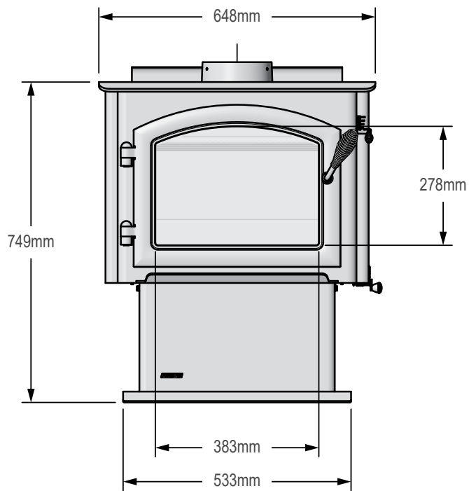
Figure 7.1 - Front View
